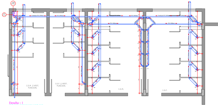
Detalhe - 1 E.S.M. I VEST. FUNCION. E.S.F. I VEST. FUNCION. E.S.M.
