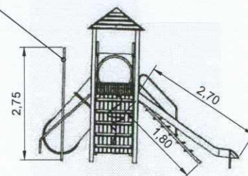
VISTA FRONTAL
