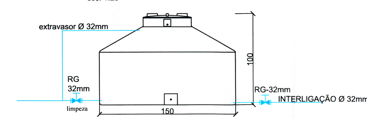
Detalhe T01, T02, T03, T05 esc. 1:25
